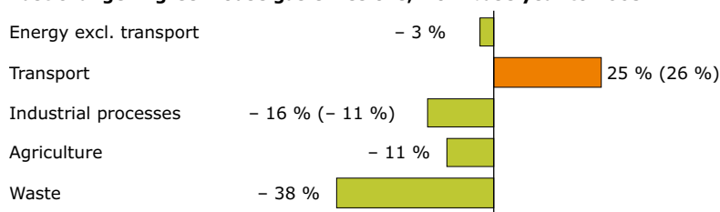
Figure 9.2 Changes in EU-15 greenhouse gas emissions by sector
