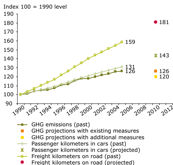
Figure 9.12 EU-15 and EU-27 greenhouse gas emissions from transport compared with transport volumes (passenger transport by car and freight transport by road) (1990–2005)
